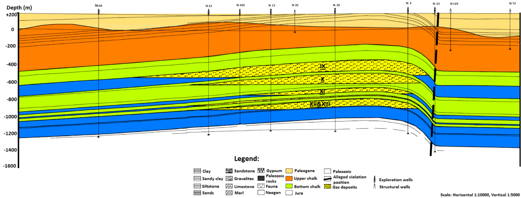
Figure 2a. Gazli field vertical cross section profile by line 1-1 as defined on Figure 1.
