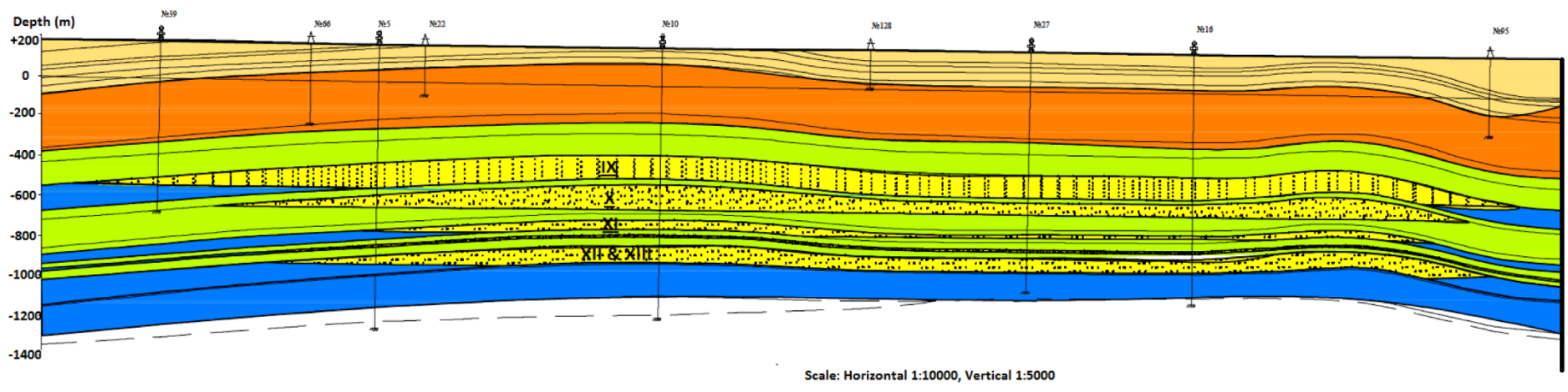
Figure 2b. Gazli field vertical cross section profile by line 2-2 as defined on Figure 1.
